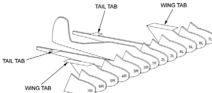
Figure 1 Fuselage Assembly
